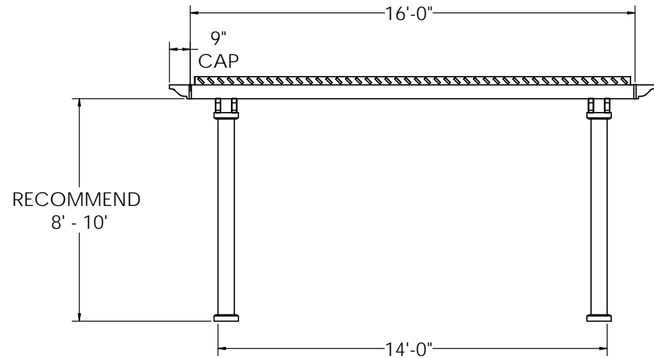
Center of Post to Structure Measurement
