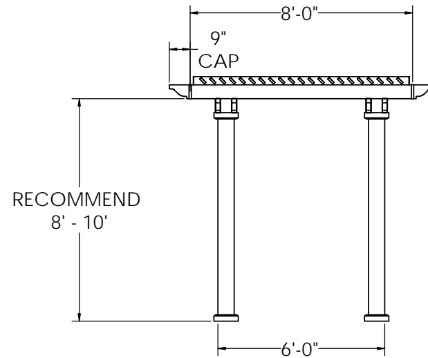
Center of Post to Structure Measurement
